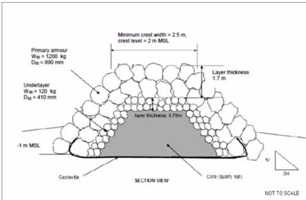
Figure 47: Diagram of a coral rock groyne
