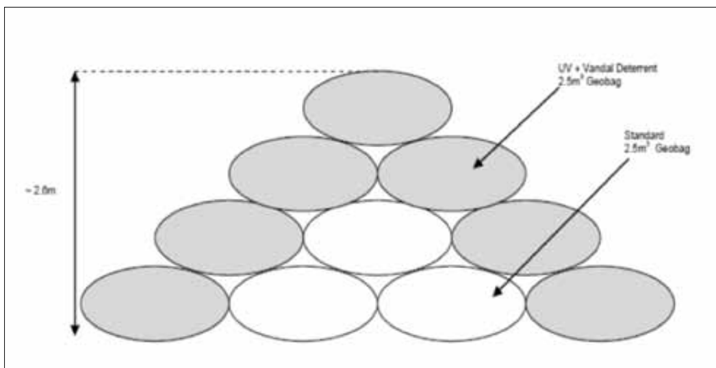
Figure 48: Design of a geotextile bag groyne
