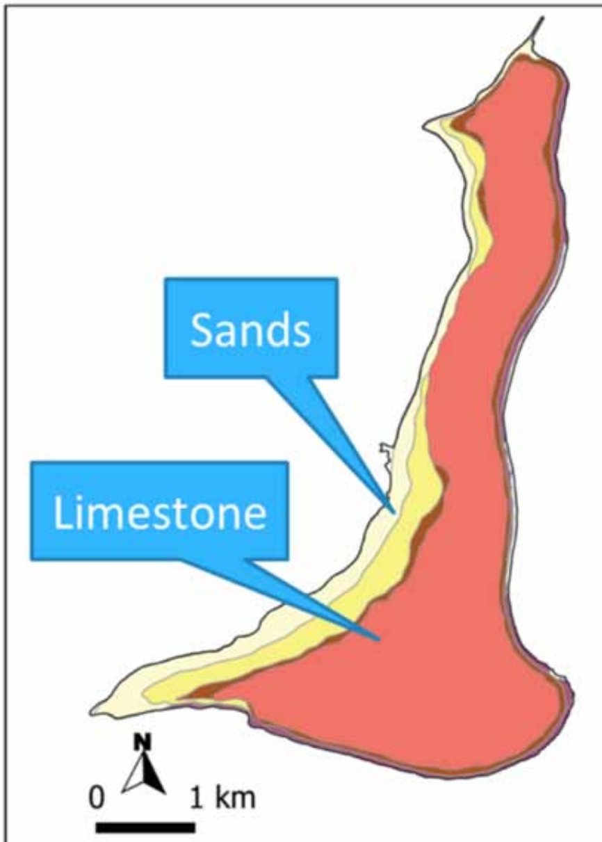
Figure 10: Simplified soils map of Lifuka. Note that the low-lying coastal plains of the western shoreline comprise unconsolidated sands.
