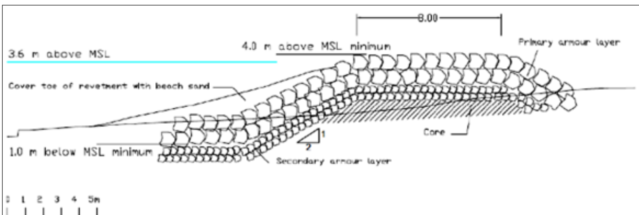
Figure 38: Example of the type of revetment that could be built at Lifuka
