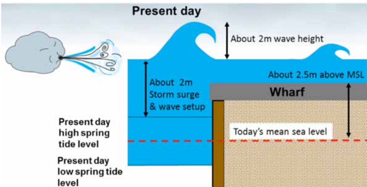
Figure 31: Schematic showing the effects of an extreme tropical cyclone storm on seas at Pangai wharf, present day
