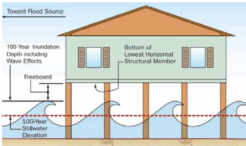
Figure 53: Source: Coastal Construction Manual, available at www.fema.gov .
