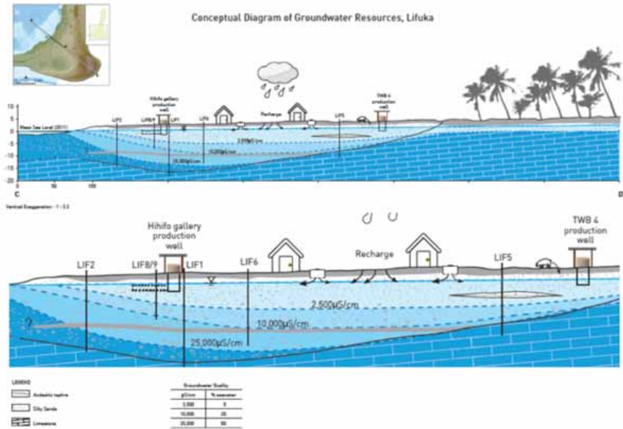
Figure 11: Conceptual diagram of groundwater resources, Lifuka
