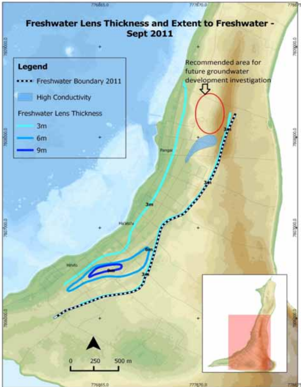
Figure 12: Extent of fresh groundwater lens, showing area with potential for further groundwater development
