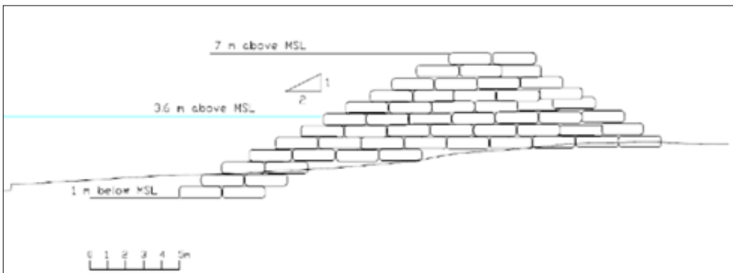
Figure 41: Example of a geotextile revetment design
