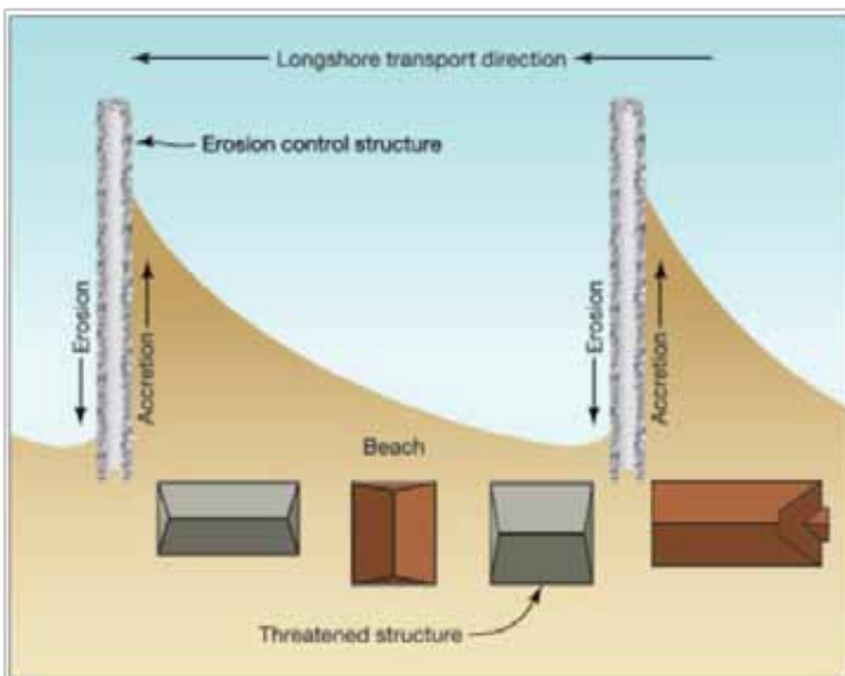
Figure 44: How groynes work
